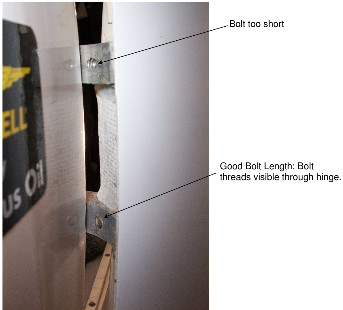
Figure 1. Hinge Bolt Detail
